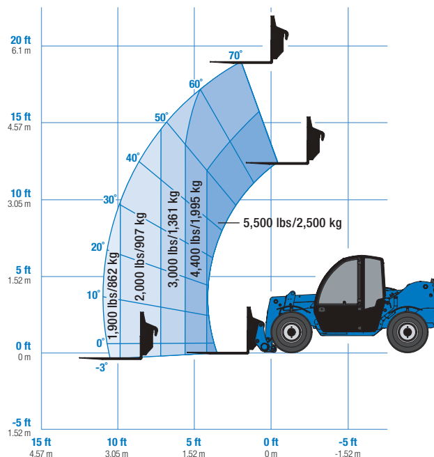
Load Chart GTH™-5519**
